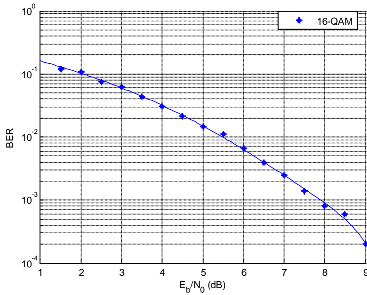
Figure 17: Bit Error Rate Performance for 16-QAM
