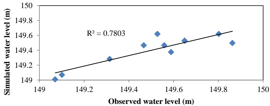
Figure 8: Comparison between simulated and observed spill elevation
