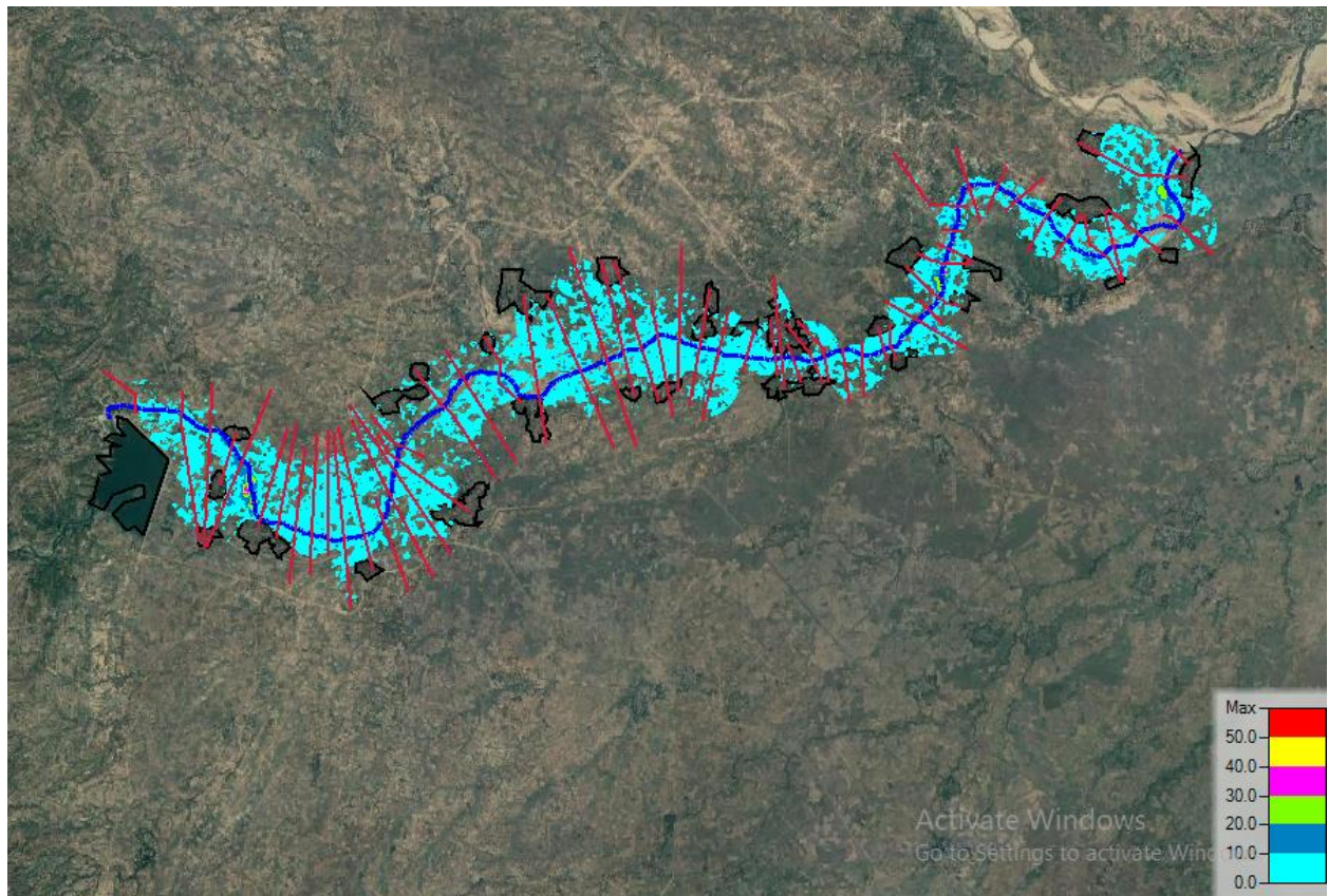
Figure 14: Flood inundation map of North Yamar dam breach by piping failure mode
