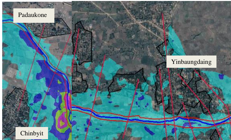
Figure 15: Flood inundation map of North Yamar dam break by piping that shows flood coverage over Padaukone, Chinbyit and Yinbaungdaing villages
