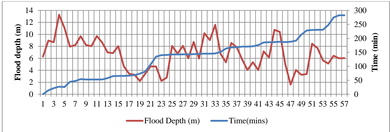
Figure 13: Maximum Flood Depth and Arrival Time for piping at bottom failure
