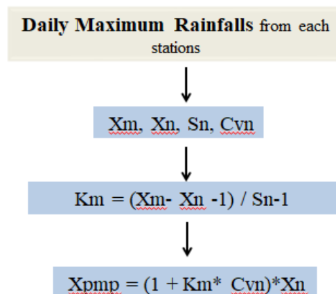
Figure 2: Workflow of PMP calculation.
