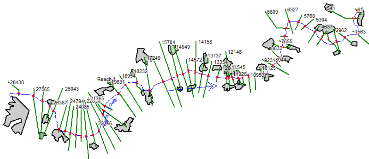
Figure 6: Geometrical view of North Yamar River in HEC-RAS
