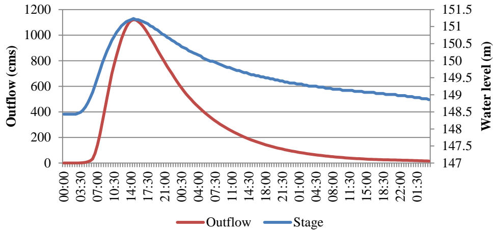
Figure 10: With emergency spillway on overtopping failure
