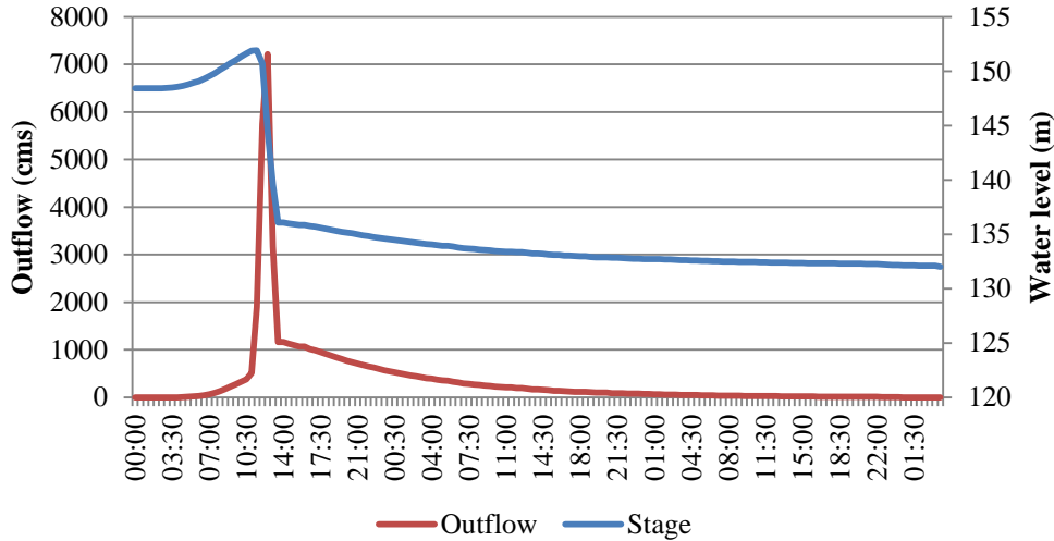
Figure 9: Without emergency spillway on overtopping failure.
