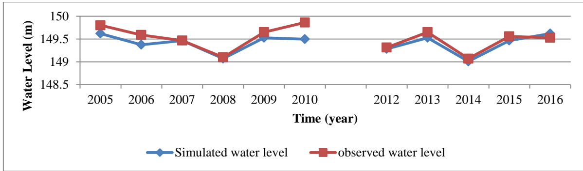
Figure 7: Comparison between simulated and observed spill elevation
