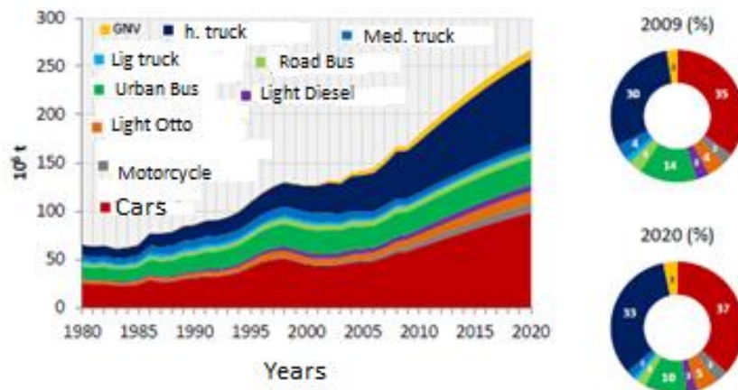
Figure 3: CO 2 emissions by vehicle category. Extracted and adapted from [6]
