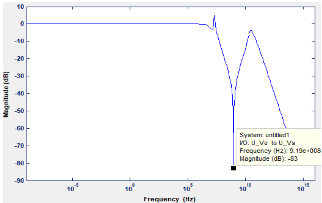
Figure 6: hybrid structure Bode diagram
