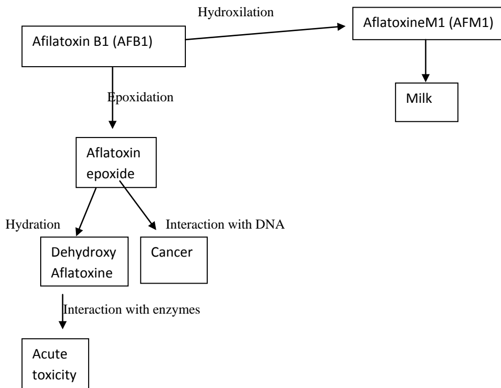
Figure 3 Some metabolic products from AFB1
