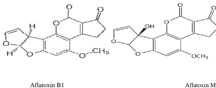
Figure 2 Chemical Structure of Aflatoxin B 1 and Aflatoxin M1
