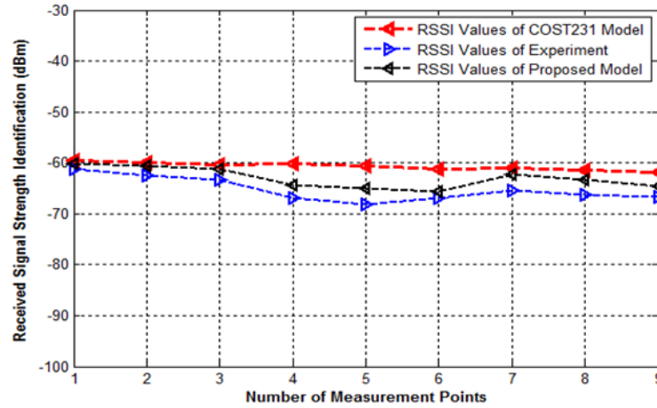
Figure 5: Comparison of RSSI Values among the COST 231, Experiment and Proposed Model of Indoor-to-Outdoor Area
