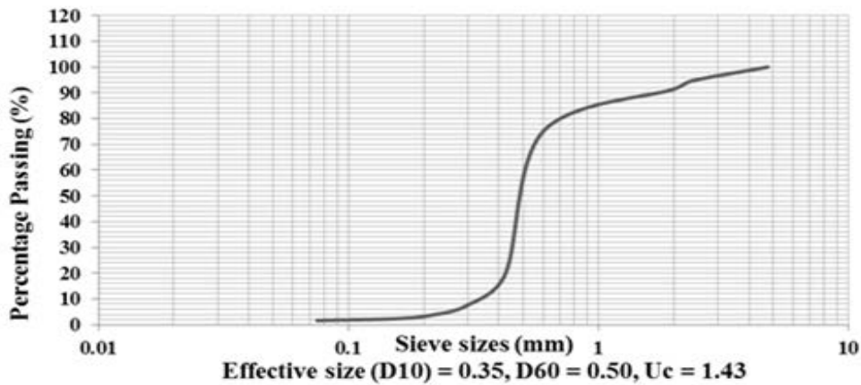
Figure 4: Particle size distribution of river benue sand.
