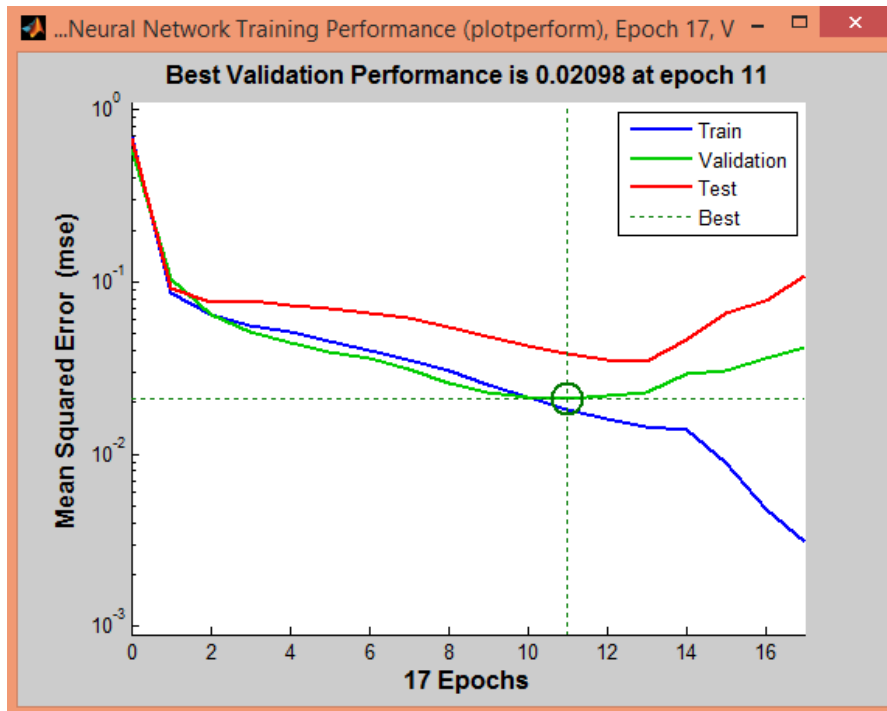
Figure 4: The network performance error during the training
