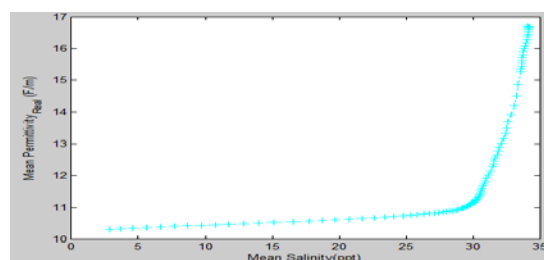
Figure 3.2 a: mean salinity vs Mean permittivity real
