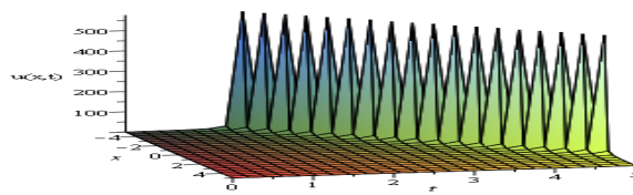
Figure 3.5: (3D Plot): Soliton profile of (3.11), when n = 2, a = 1, b = 1, c_1 = 1
