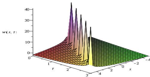
Figure 3.1: (3D Plot): Profile of (3.9),
