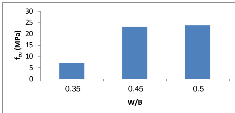
Figure 1b.i: Effect of W/B on Compressive Strength for FA/MS = 0 (control)
